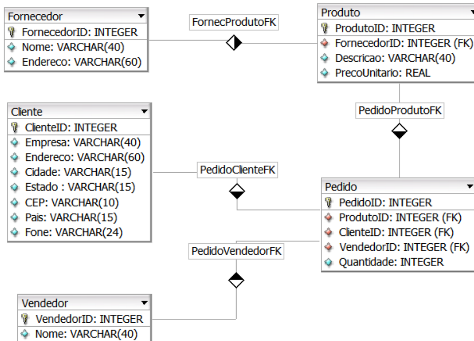
Figure 1 – Diagrama relacional.
