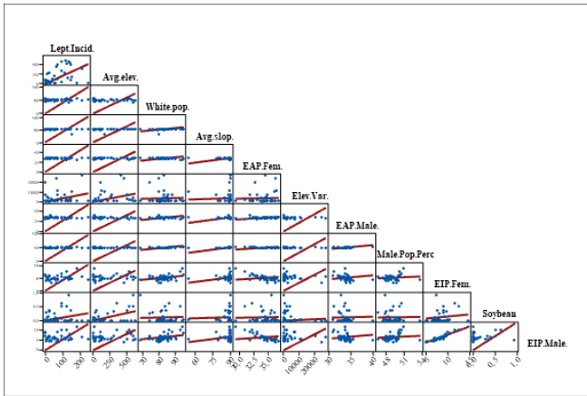
Figure 10: Example of a scatter plot between leptospirosis incidence and the ten variables with the highest Spearman correlation for Group 1 of predominantly rural flooded areas.
