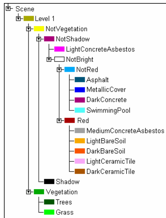
Figure 1 – Semantic Network
