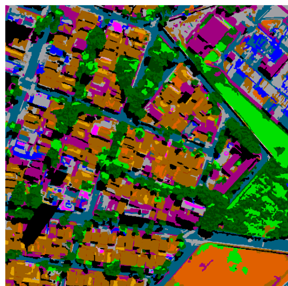
Figure 2 – Classification Results
