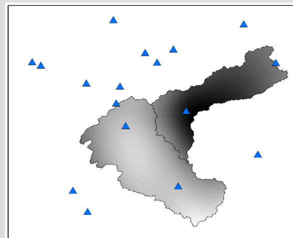
Spline
