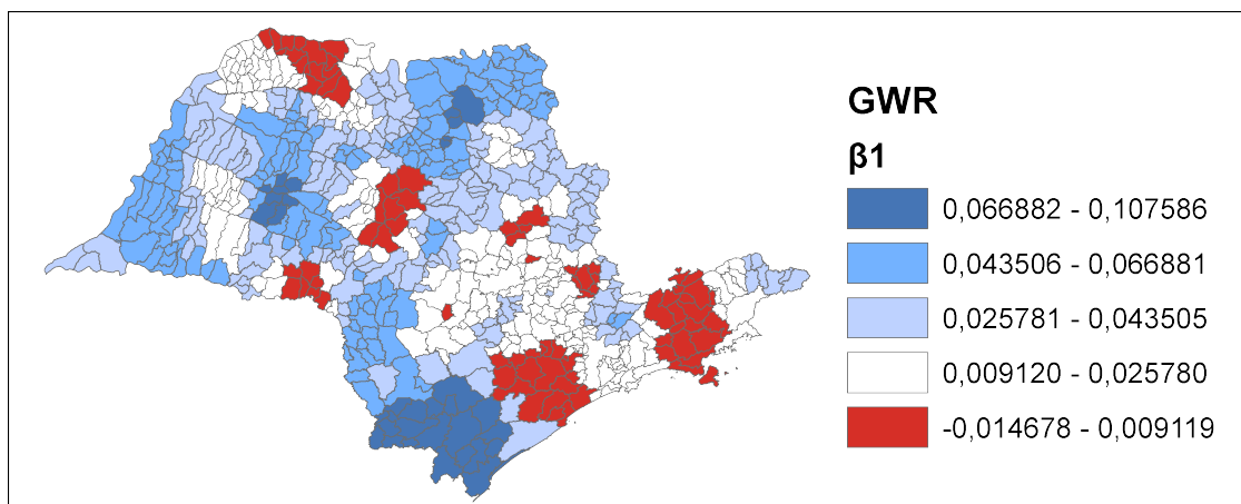
Figura 9: Coeficiente angular \beta_1
