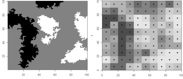
Figure 2. Left side: zones image of the dataset in Figure 1. Right side: geosensor data and the network's nodes.
