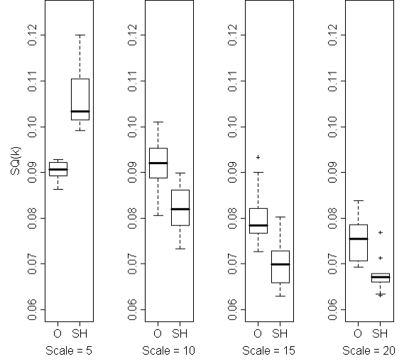
Figure 3. Boxplots for SQ_k values.
