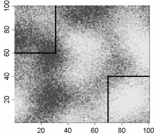
Figure 1. Spatial distribution of luminosity measurements
